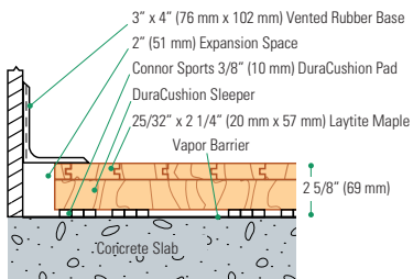
Wall Base Detail
