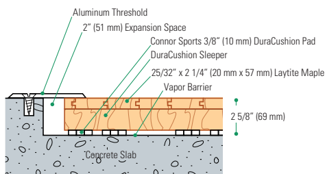
Threshold Detail (Optional Accessory)
