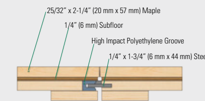
TONGUE & GROOVE DETAIL
