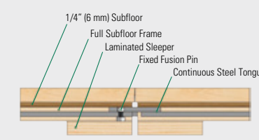
FUSION PANEL CONNECTION
