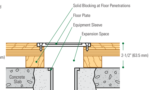
Equipment Detail ( Optional Accessory )
