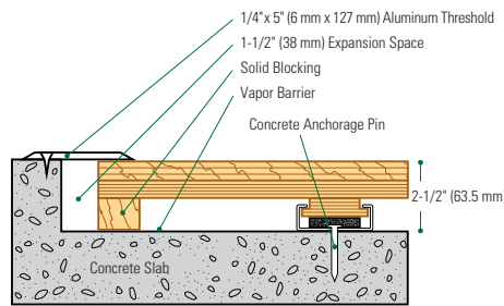
Threshold Detail ( Optional Accessory )
