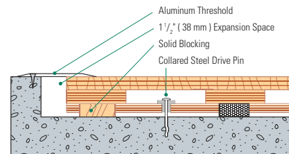
Slab Depression: 25/32" (20 mm) flooring - 2 1/4" (57 mm)
