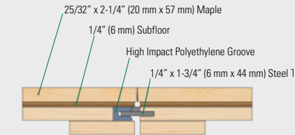
TONGUE & GROOVE DETAIL
