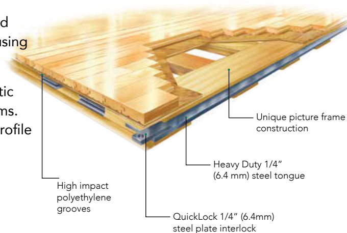
FUSION PANEL CONNECTION
