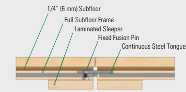
FUSION PANEL CONNECTION
