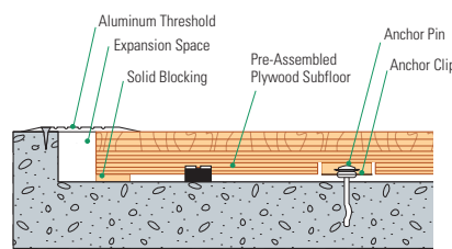
Slab Depression: 25/32" (20 mm) flooring - 1 1/4" (44 mm)
