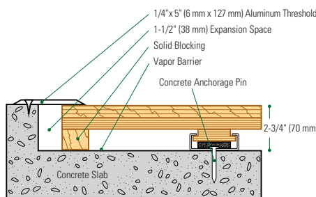
Threshold Detail ( Optional Accessory )
