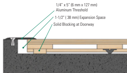
Threshold Detail (Optional Accessory)
