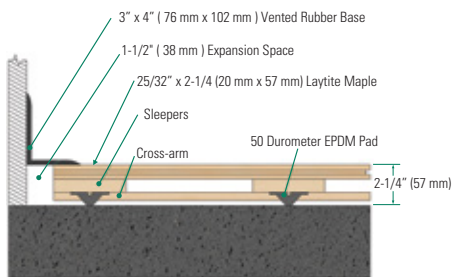
Wall Base Detail
