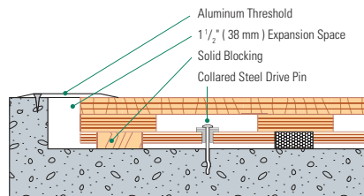
Slab Depression: 25/32" (20 mm) flooring - 2 1/4" (57 mm)
